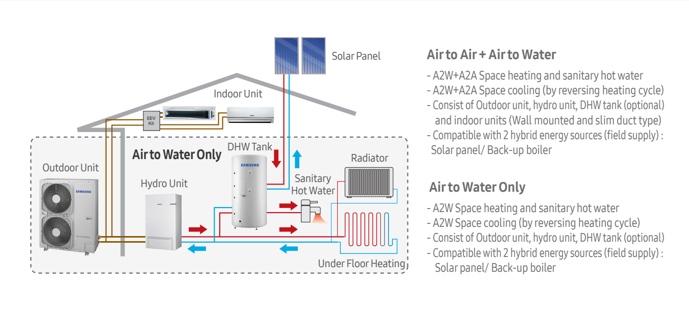
EHS TDM process (Air-to-Air and Air-to-Water)
