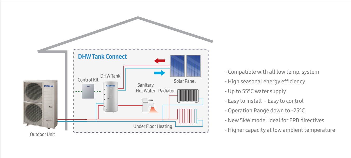
EHS Mono process overview (air-to-water)
