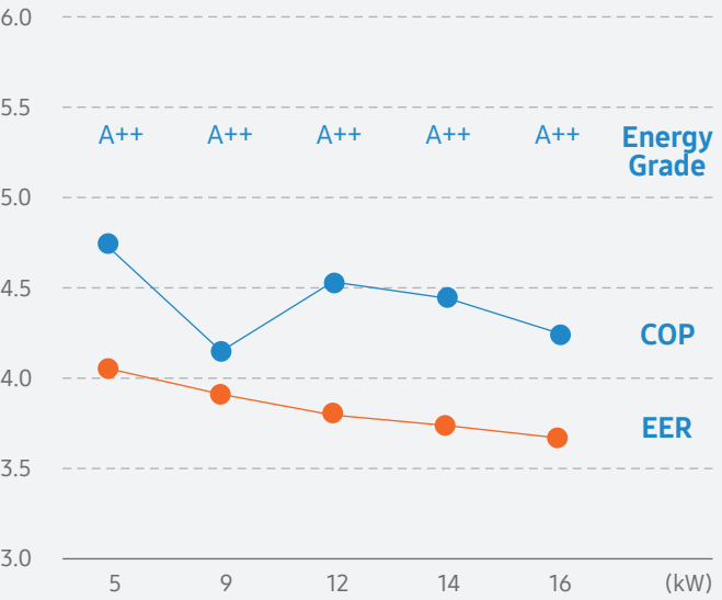
Efficiency (EHS MONO)
