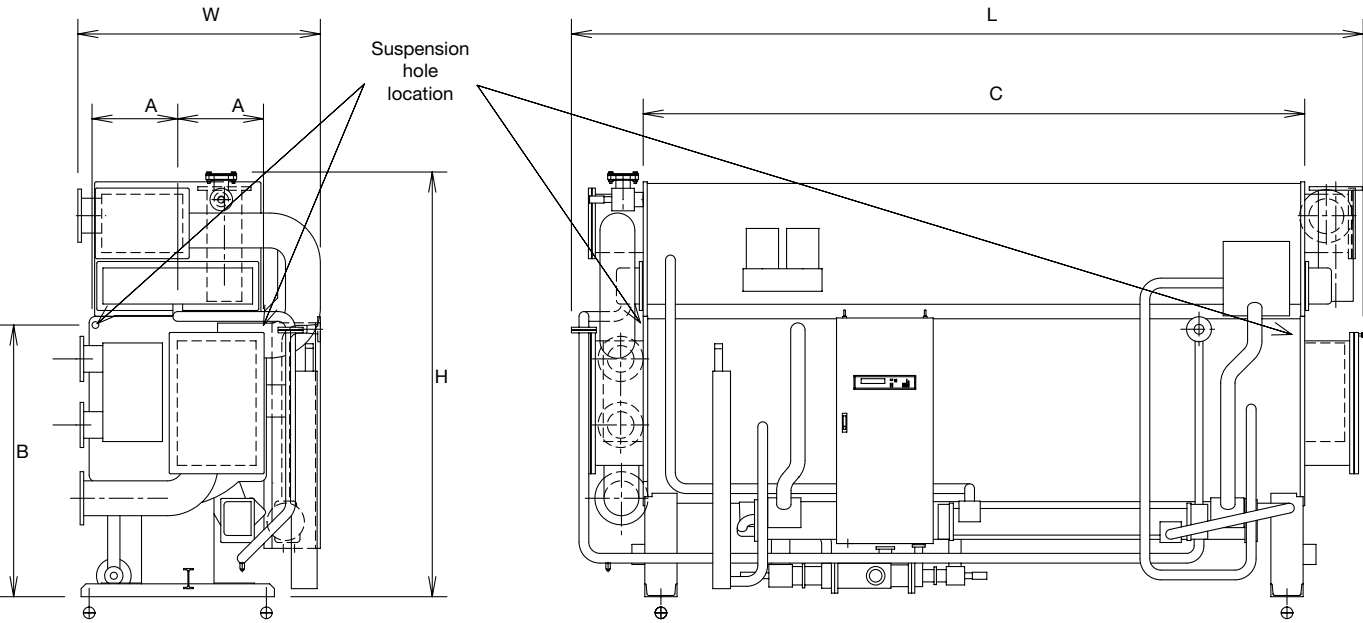
Fig. 12 - One-piece shipping
