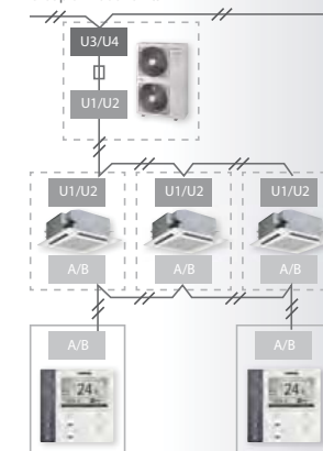
Group of Indoor Units
